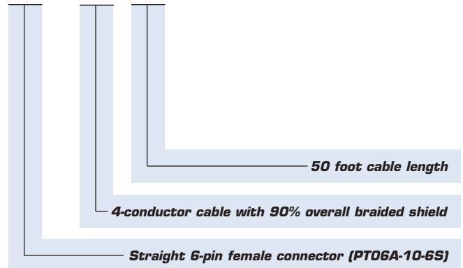
Bx6SM - BeN4 (50) (Load cell cable with tinned pig tail ends)
