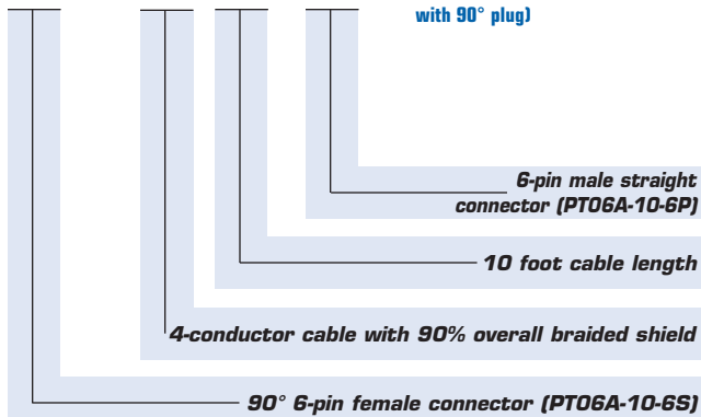
Bx6SML - BeN4 (10) - Bx6PM (Interconnecting cable assembly with 90° plug)
