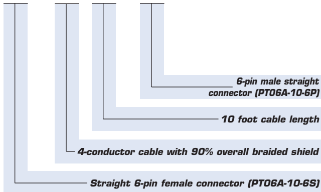
Bx6SM - BeN4 (10) - Bx6PM (Interconnecting cable assembly)
